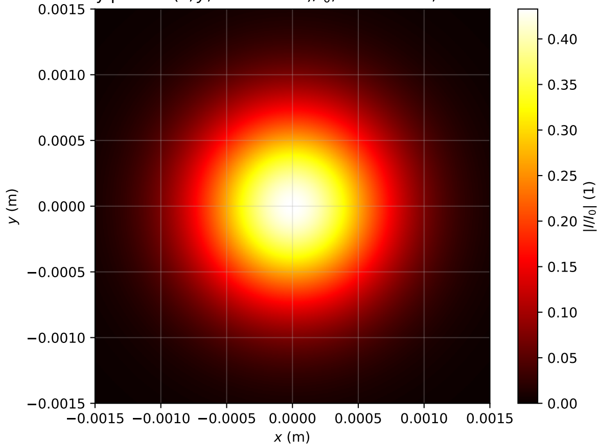
Intensity profile I(x, y, z = 2.946m)/I_0 , P_{in}=0.3P_{cr} , artificial time
